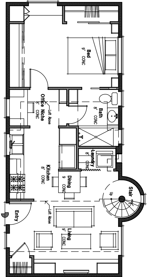
LOWER FLOOR
