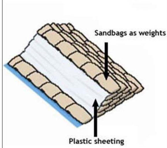
Additional waterproofing
