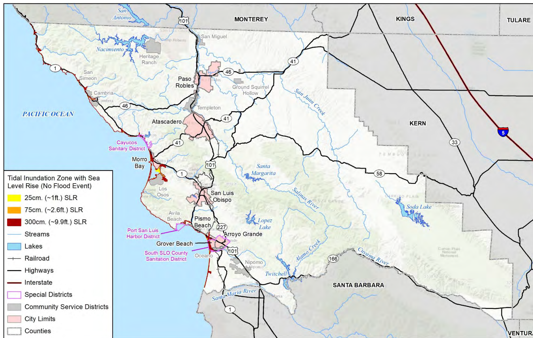
Figure 5-33 Sea Level Rise Scenario Analysis: Tidal Inundation Only
