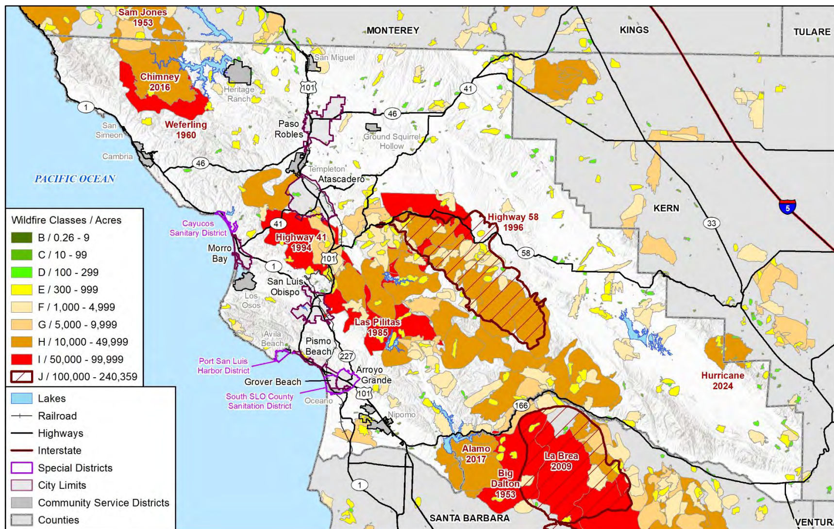
Figure 5-96 Wildfires in San Luis Obispo County from 1912 to 2024
