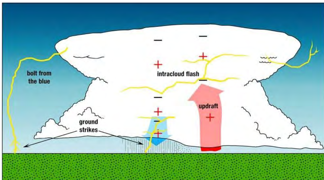
Figure 5-8 Cloud to Ground Lightning
