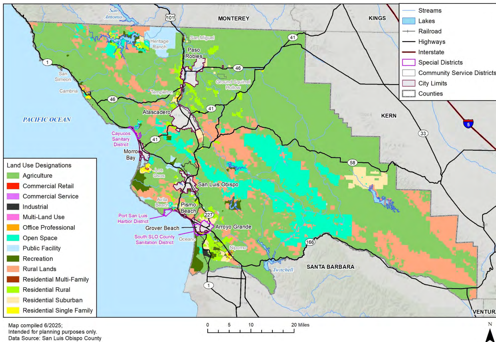
Figure 5-24 San Luis Obispo – County Land Use
