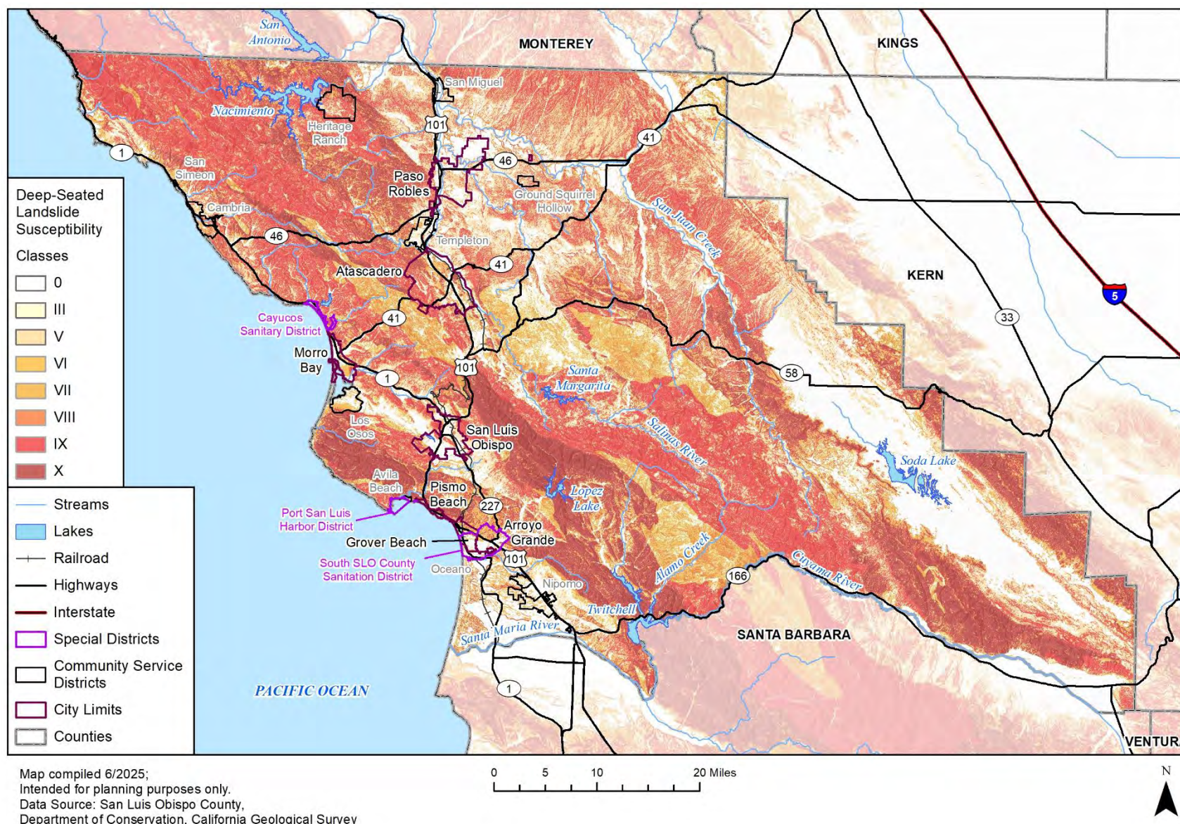
Figure 5-87 Landslide Potential
