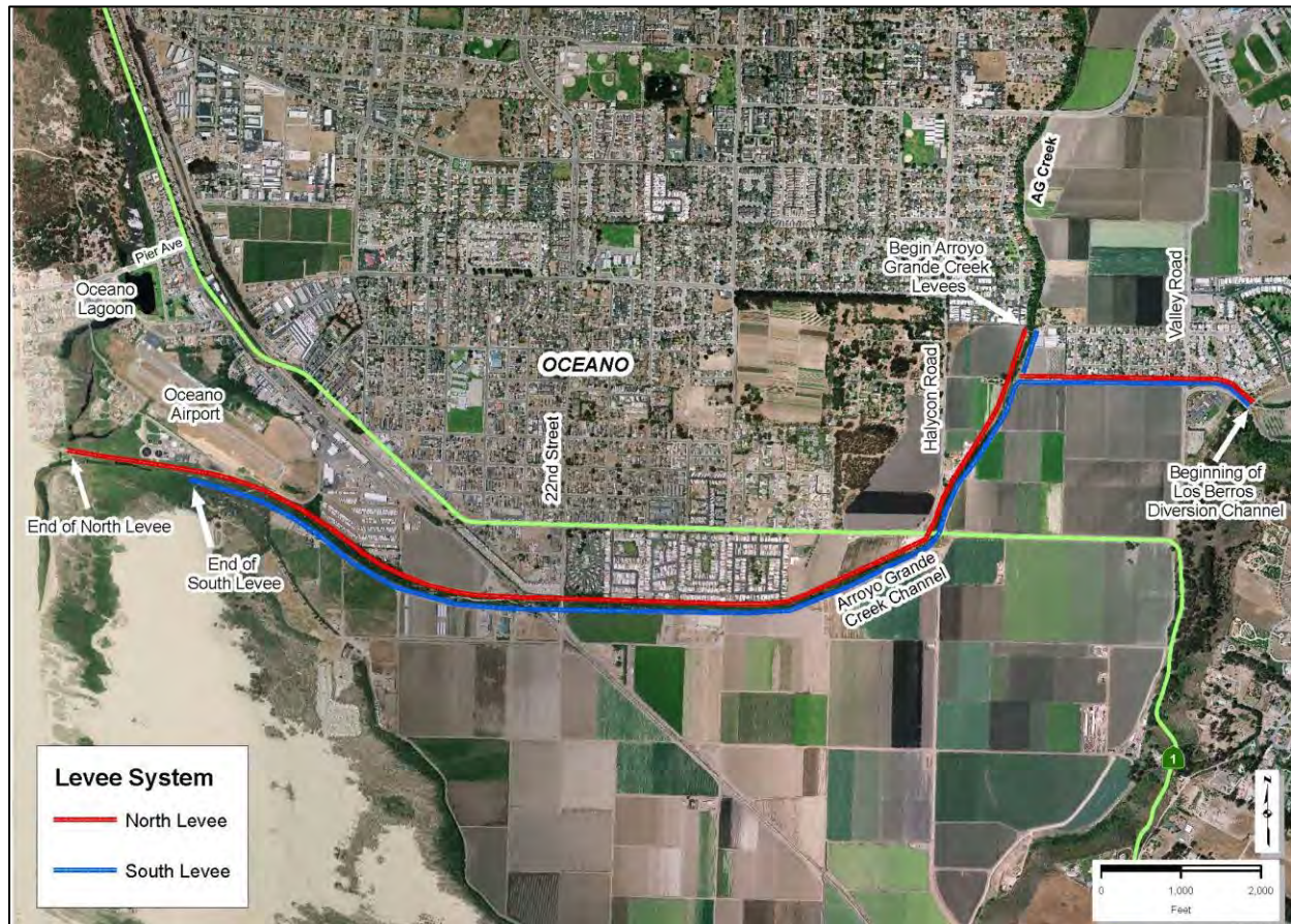
Figure 5-75 Arroyo Grande Creek Levee System
