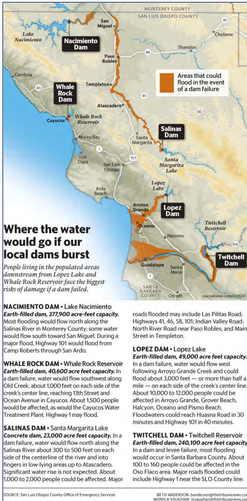
Figure 5-51 Dam Inundation Impacts to Downstream Communities in San Luis Obispo County
