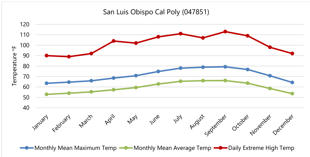
Figure 5-15 San Luis Obispo Poly Tech Daily Temperature Averages and Extremes (Period of Record 1927-2024)
