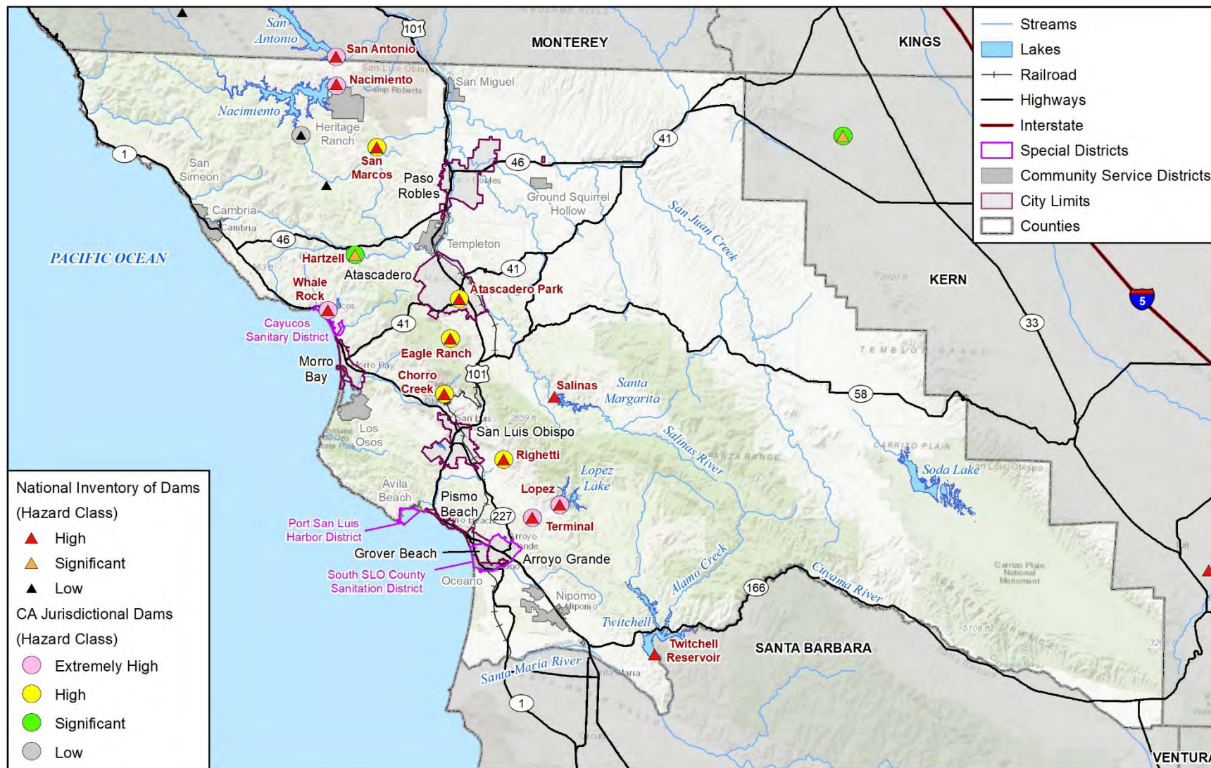
Figure 5-48 Dams of Concern to San Luis Obispo County
