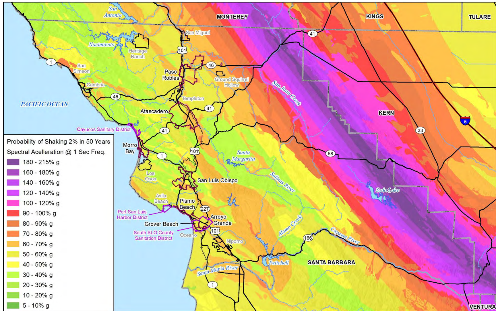
Figure 5-64 Ground Shaking Potential from Spectral Acceleration the Planning Area - Probability of Shaking 2% in 50 Years
