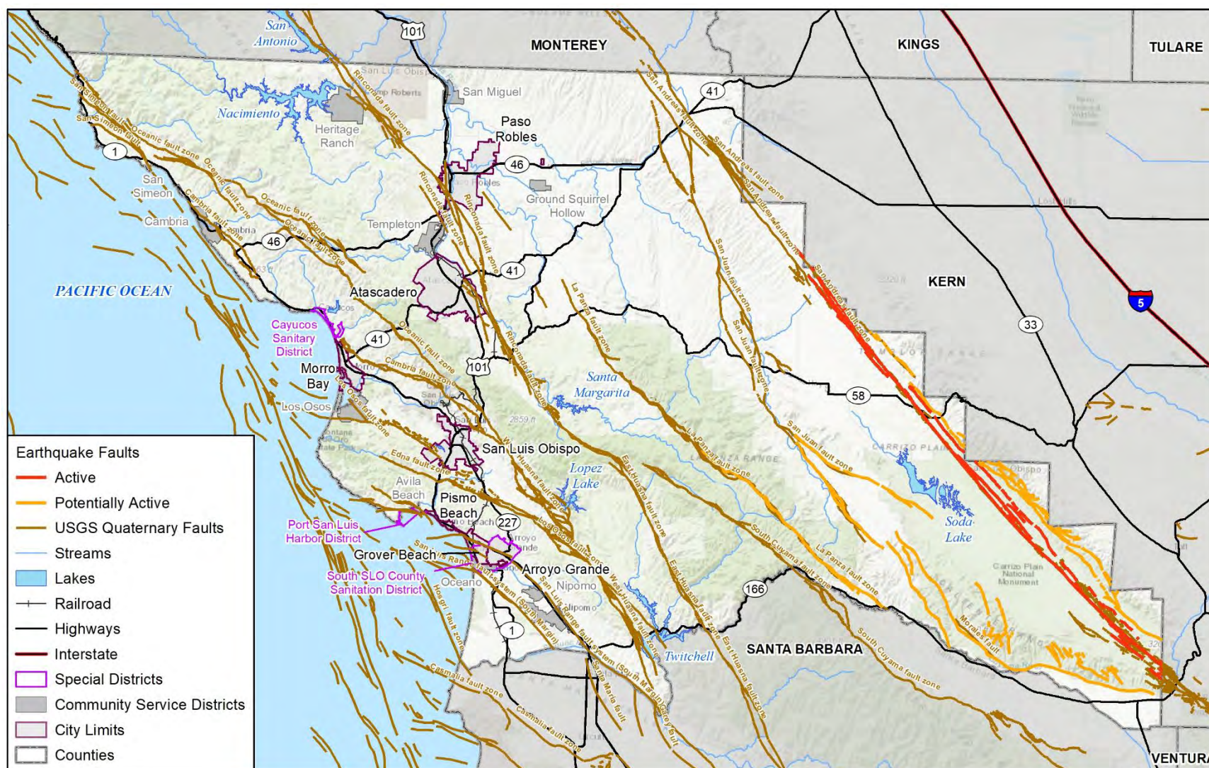
Figure 5-63 Earthquake Faults and Active/Potentially Active Faults
