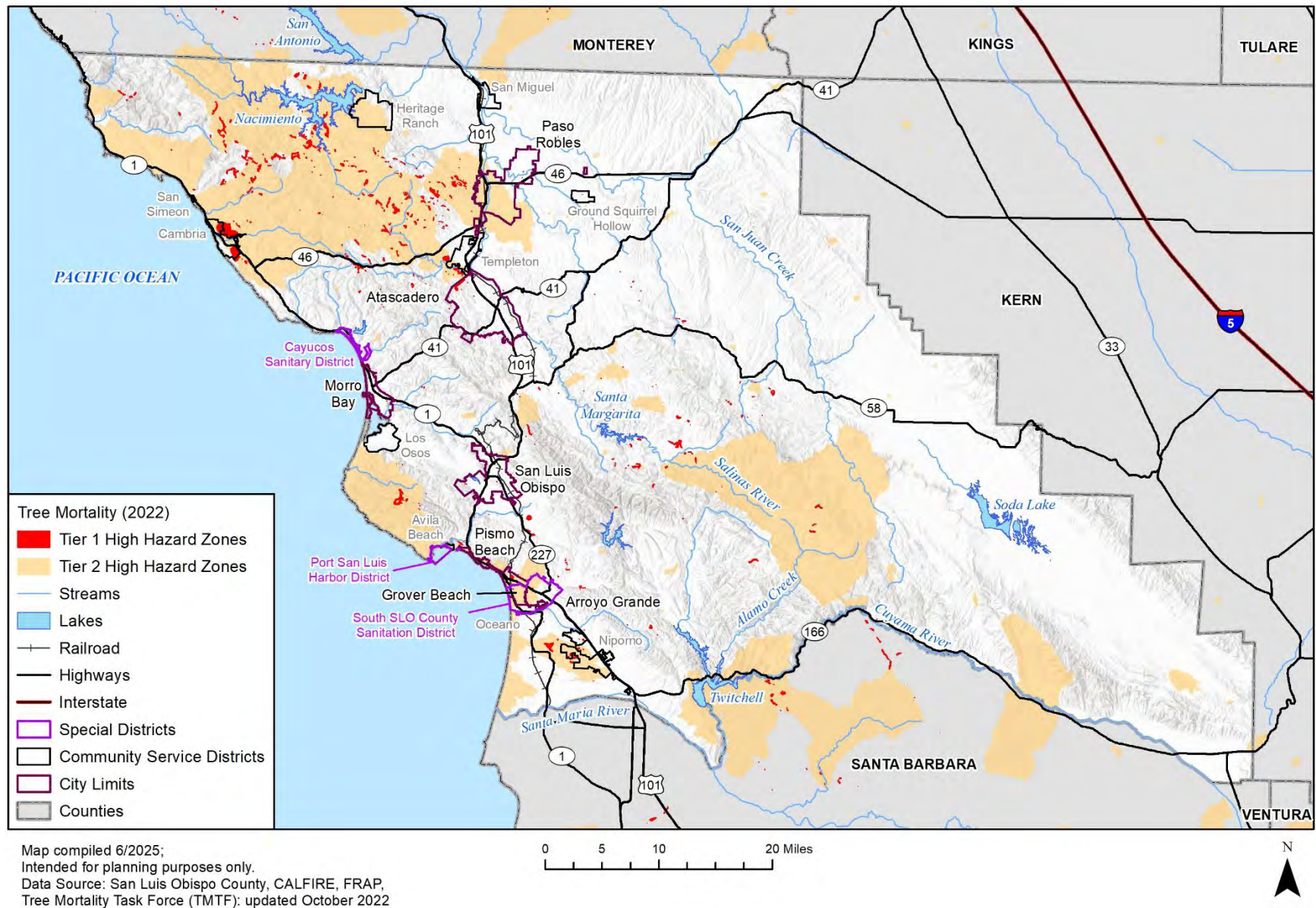
Figure 5-25 San Luis Obispo – Tree Mortality and High Hazard Zone
