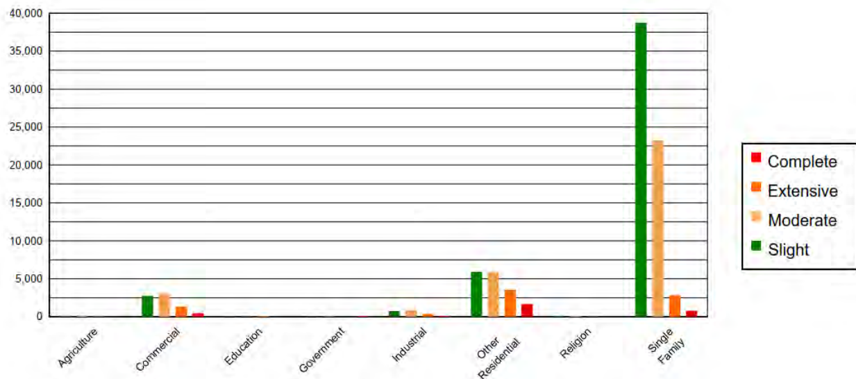
Figure 5-70 Hazus 2,500 Probabilistic Earthquake Scenario Structure Damage by Occupancy Type
