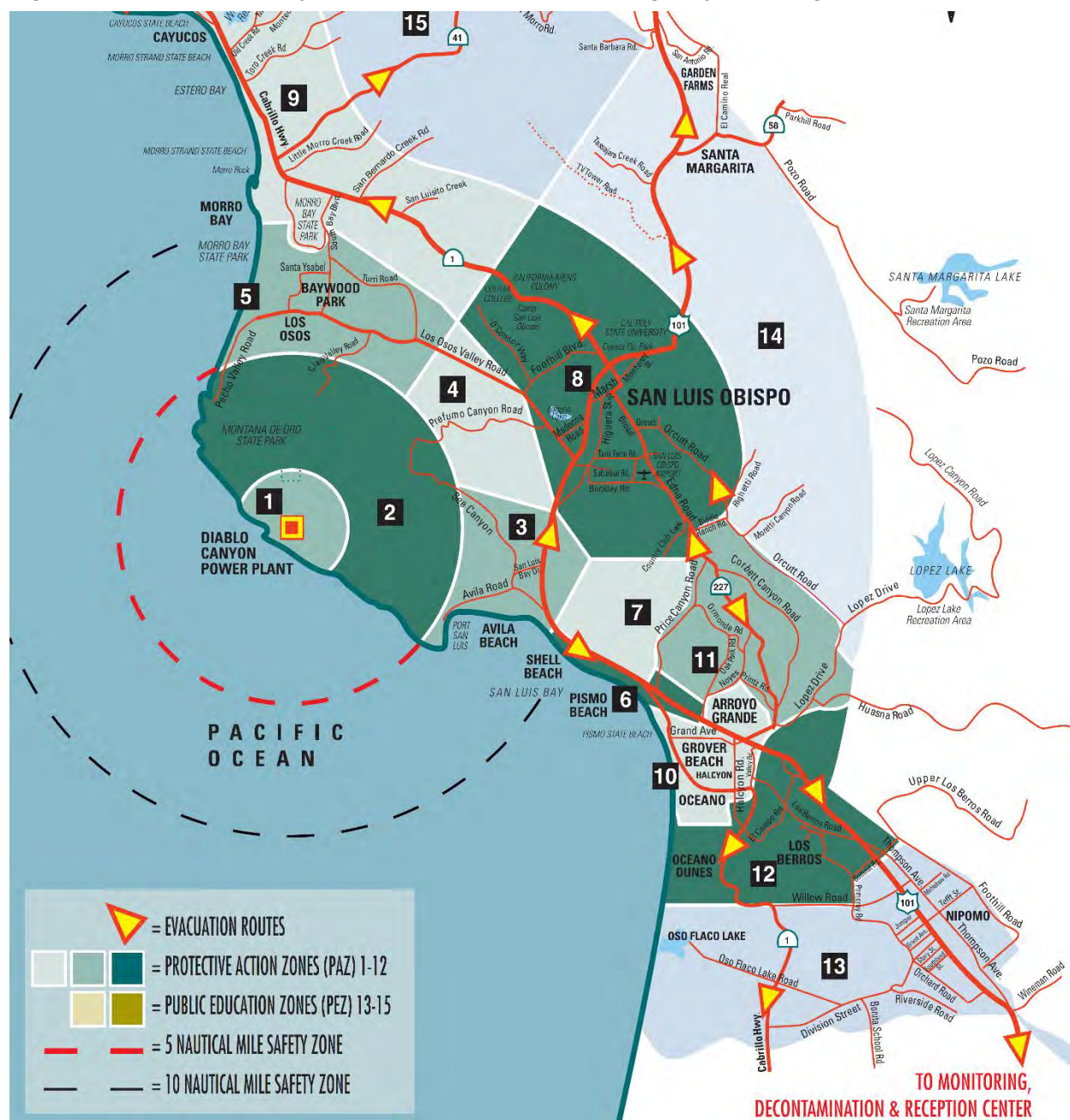
Figure 5-99 Diablo Canyon Nuclear Power Plant Emergency Planning Zones
