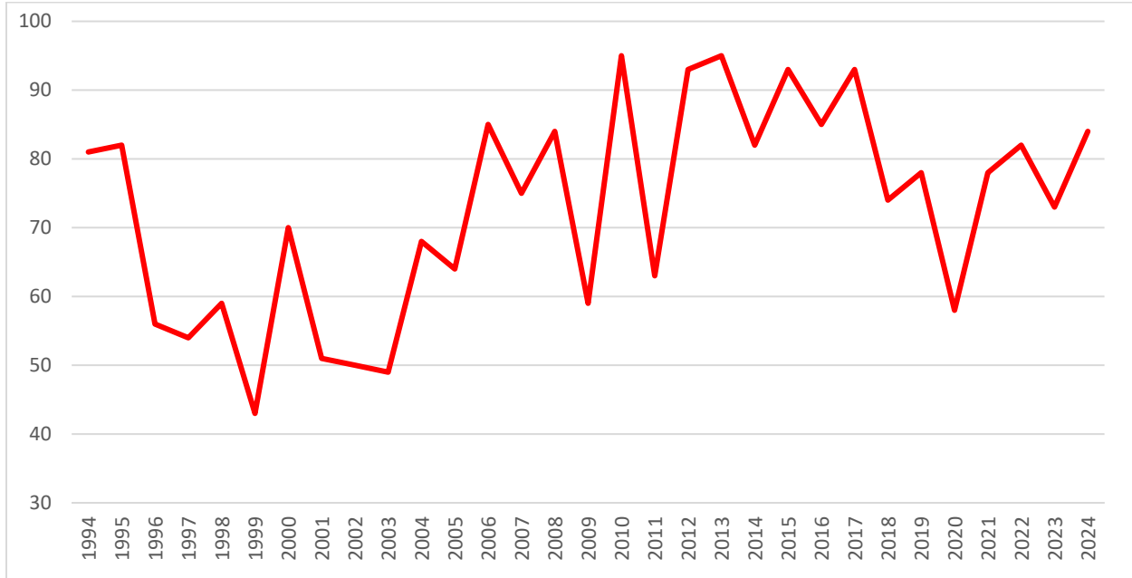
Figure 5-100 Hazardous Materials Incidents in San Luis Obispo County, 1994-2024
