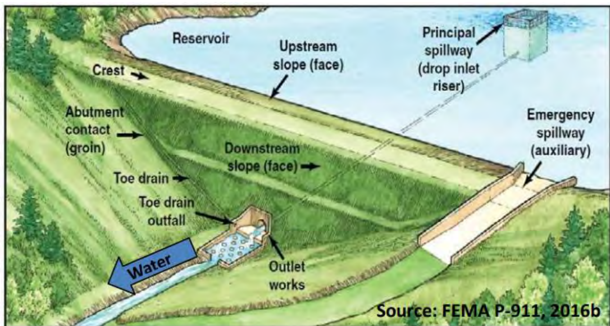
Figure 5-47 Components of a typical earthen dam (example shows earthen dam)
