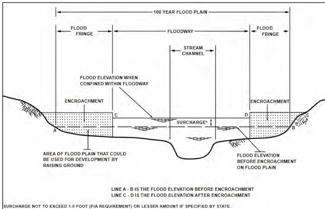
Figure 5-74 Floodplain Schematic
