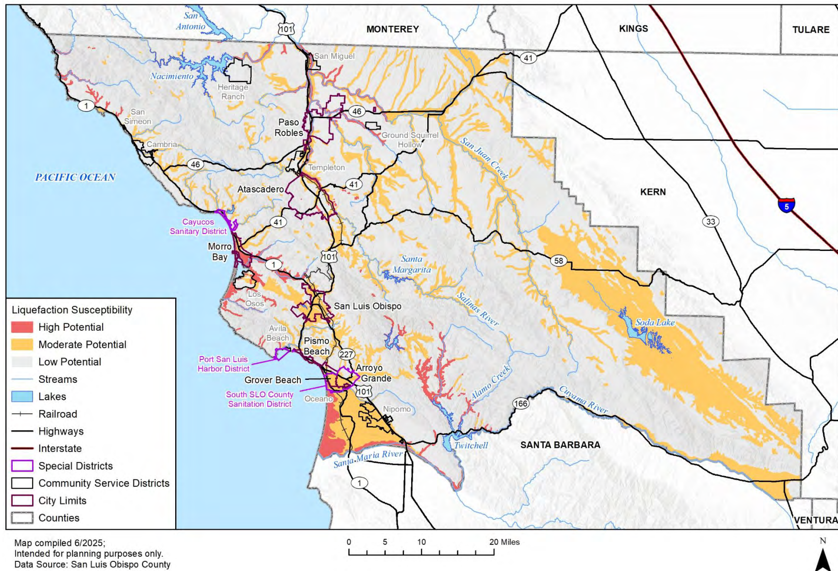
Figure 5-66 Liquefaction Susceptibility in San Luis Obispo County
