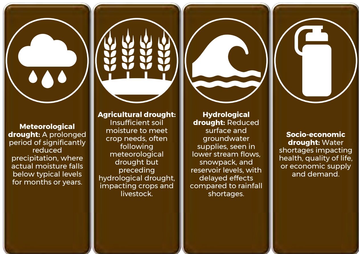
Figure 5-52 Types of Droughts
