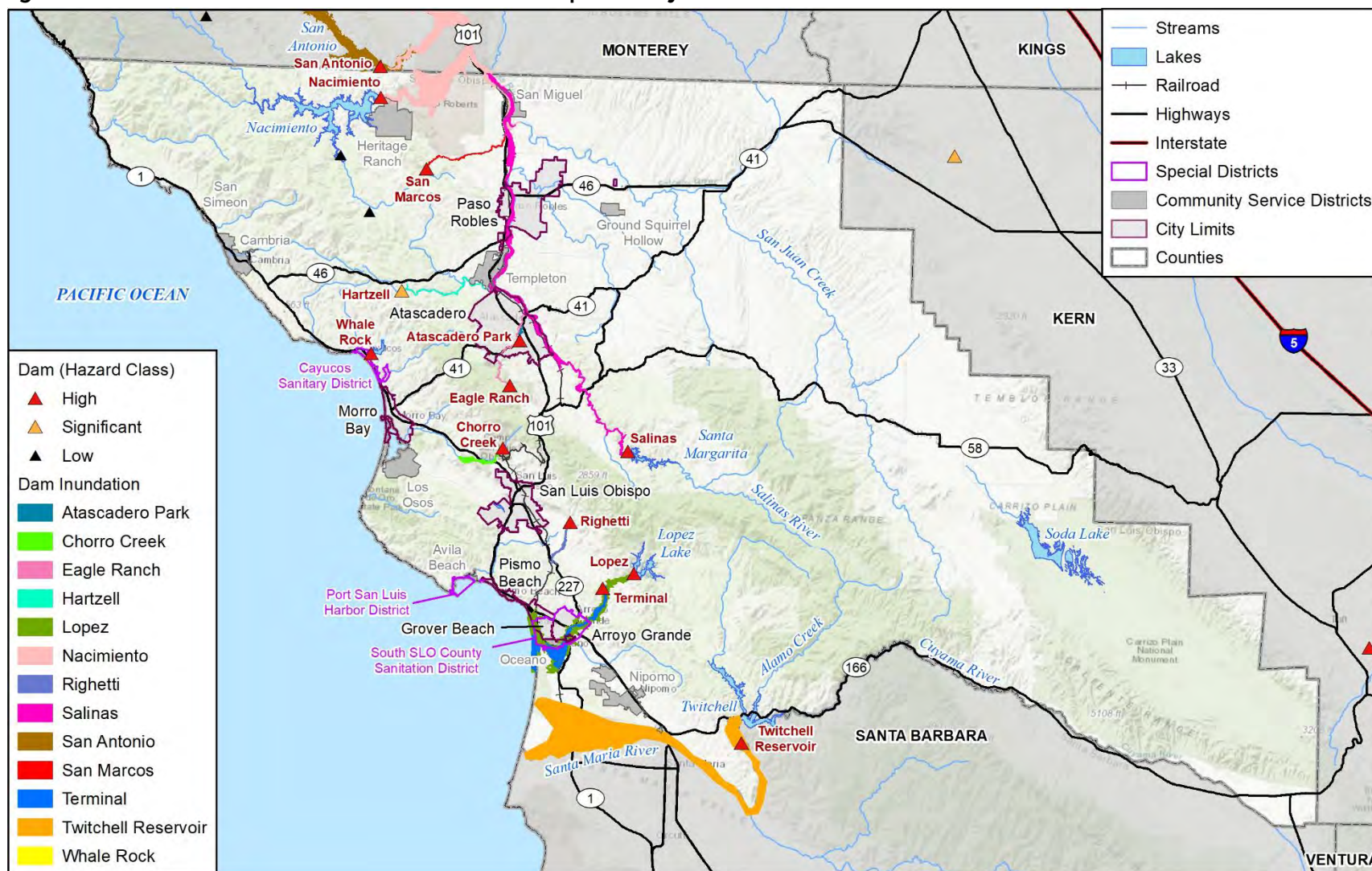
Figure 5-49 Dam Inundation Areas in San Luis Obispo County
