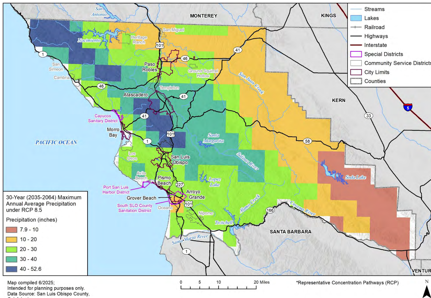
Figure 5-14 San Luis Obispo County 30-Year (2035-2064) Maximum Annual Average Precipitation under RCP 8.5
