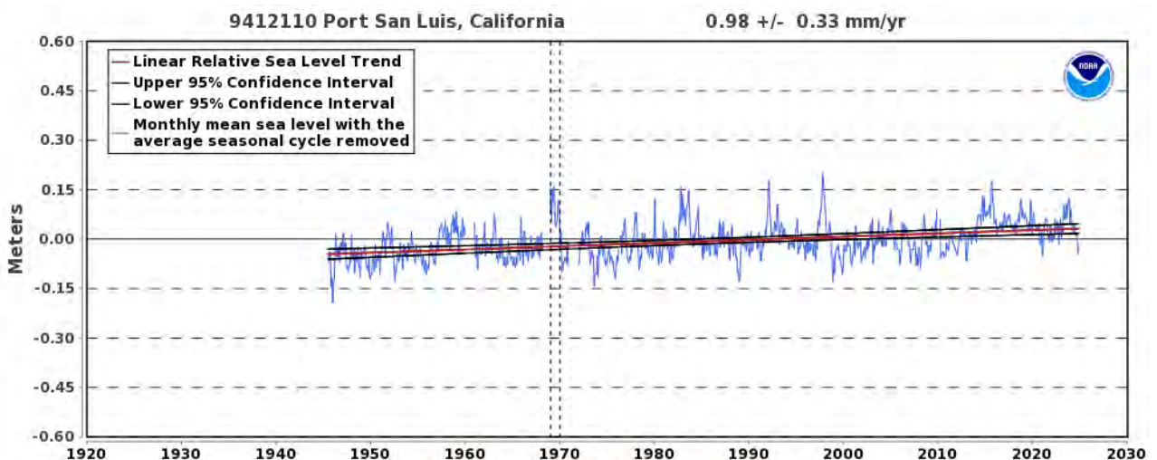
Figure 5-41 Tide Record and Sea Level Rise Trend from Port San Luis Tide Gauge (NOAA Station 9412110)
