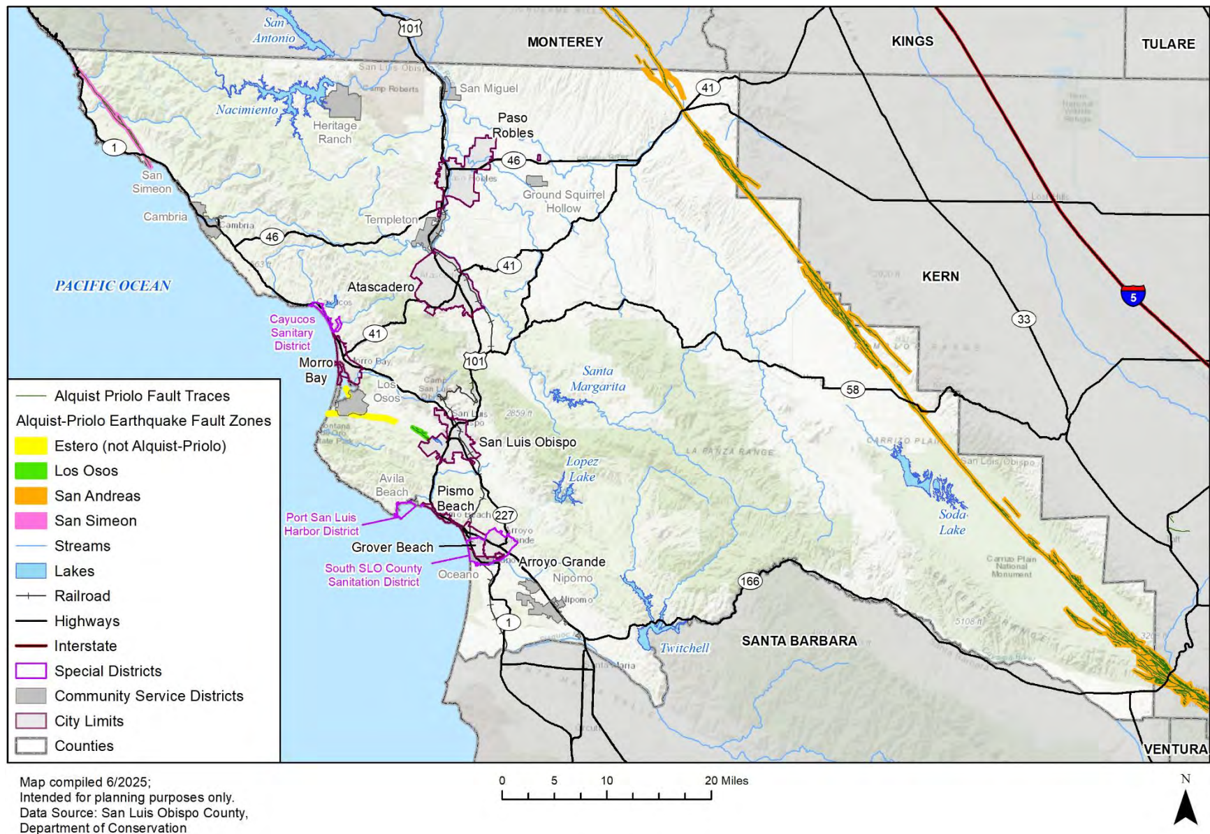
Figure 5-65 San Luis Obispo County Alquist-Priolo Earthquake Fault Zones
