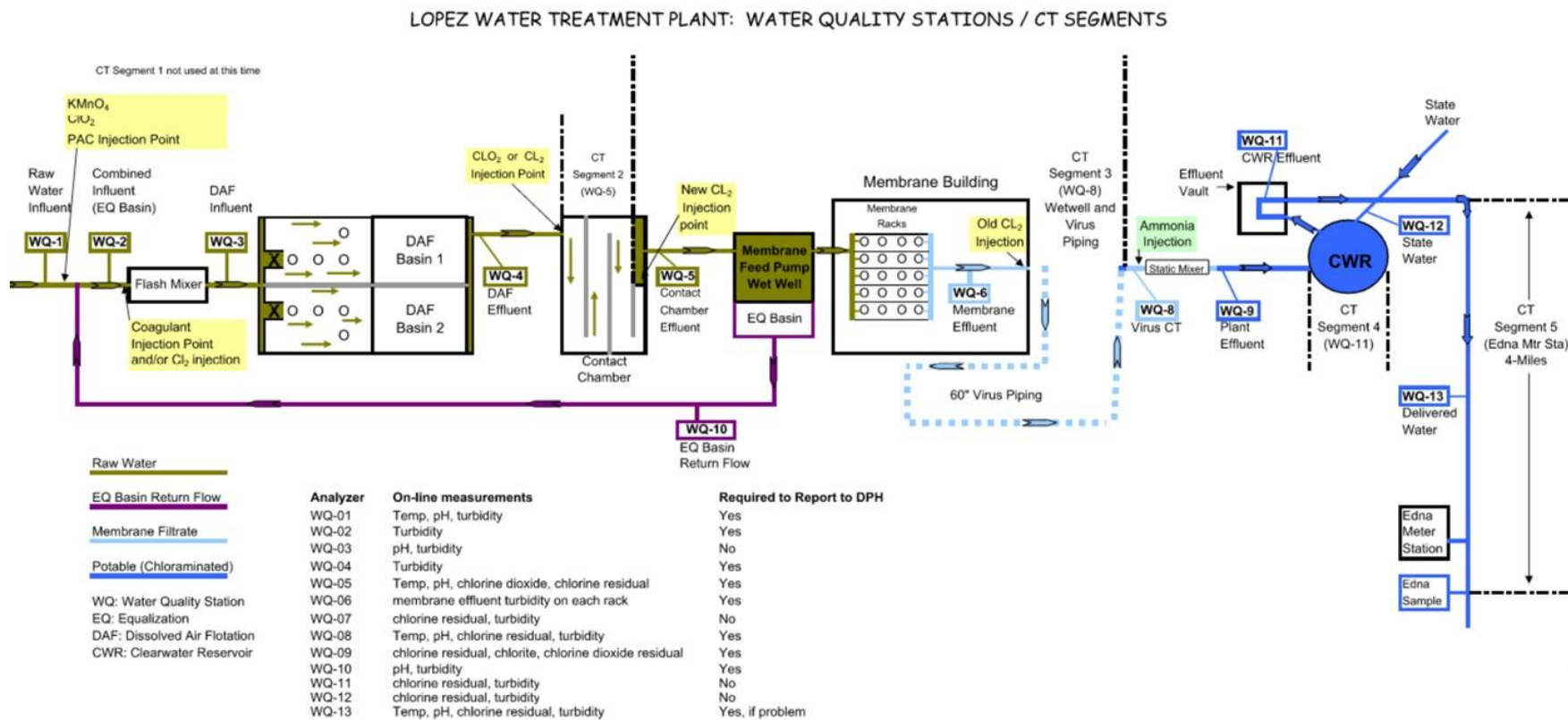
Figure 6-1. Lopez Water Treatment Plant Process Flow Diagram
